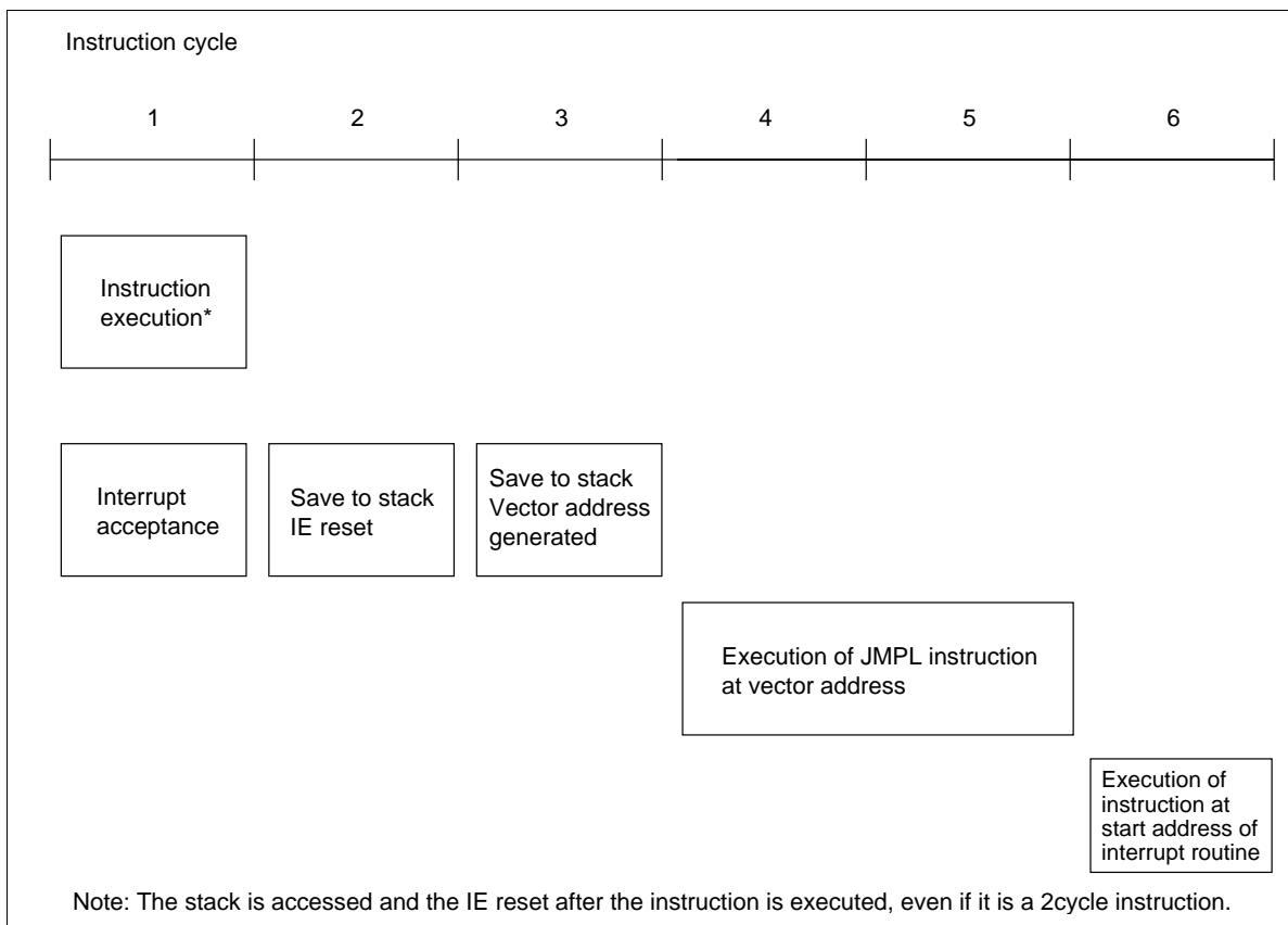
Figure 9 Interrupt Sequence
